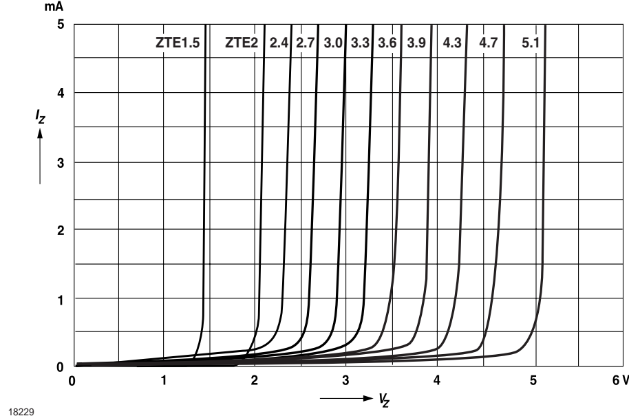
Figure 4. Breakdown Characteristics
