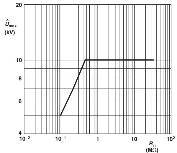
Maximum allowed peak pulse voltage in accordance with IEC 60065, 14.1.a); 50 discharges from a 1 nF capacitor charged to Umax.; 12 discharges/min (drift ΔR/R ≤ 2 %)
