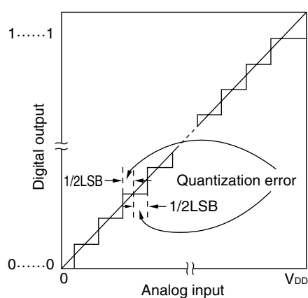
Figure 9-14. Quantization Error
