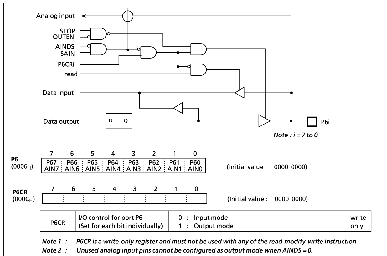
Figure 2-6. Port P6
