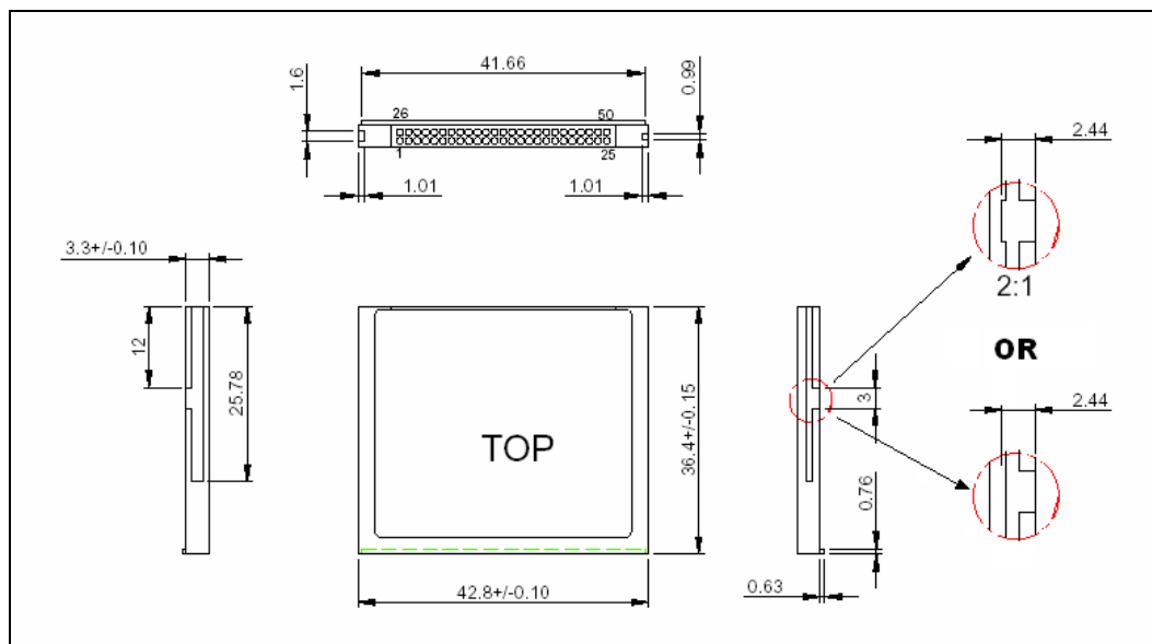
Figure 2-1. Physical Dimensions
