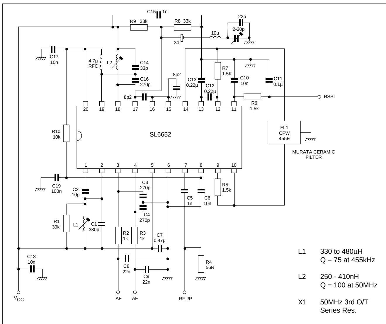
Fig. 17 Circuit diagram of SL6652 application circuit
