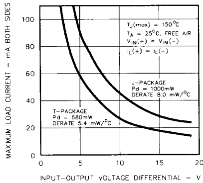
FIGURE 3. MAXIMUM CURRENT CAPABILITY
