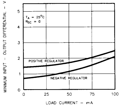
FIGURE 2. REGULATOR DROPOUT VOLTAGE
