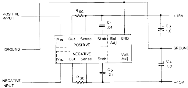
FIGURE 14 - BASIC ±15 V, 50mA REGULATOR
