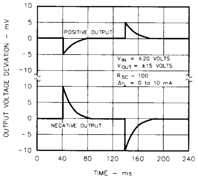
FIGURE 10. LOAD TRANSIENT RESPONSE
