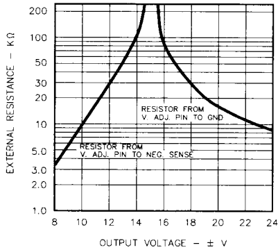
FIGURE 7. EXTERNAL PARALLEL RESISTOR REQUIRED FOR VOLTAGES OTHER THAN \pm 15 VOLTS
