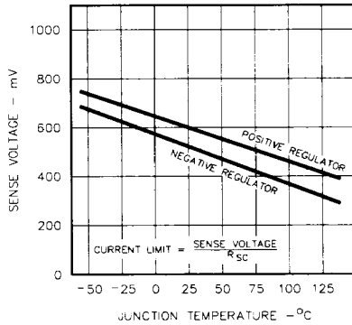
FIGURE 4. CURRENT LIMITING CHARACTERISTICS
