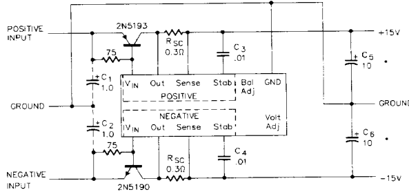
FIGURE 13 - HIGH CURRENT CONFIGURATION, ONE AMP OUTPUT
