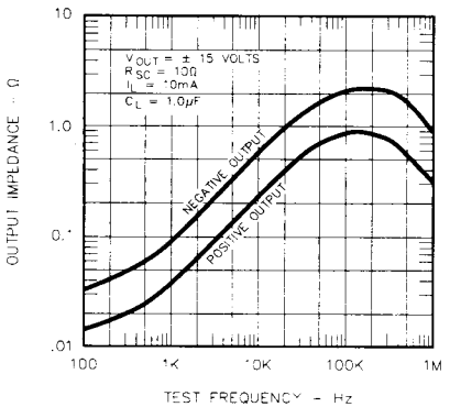
FIGURE 12. OUTPUT IMPEDANCE
