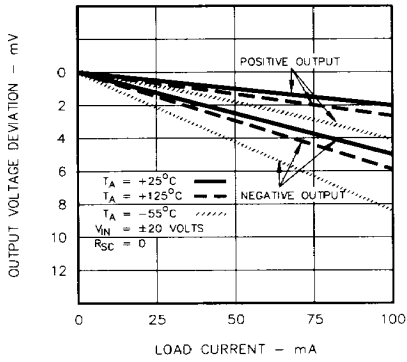
FIGURE 1. LOAD REGULATION
