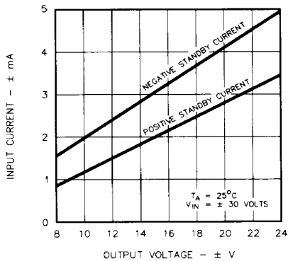
FIGURE 6. STANDBY CURRENT DRAIN
