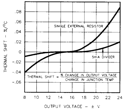
FIGURE 8. TEMPERATURE COEFFICIENT OF OUTPUT VOLTAGE
