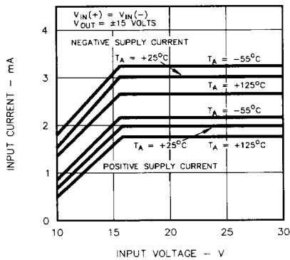
FIGURE 5. STANDBY CURRENT DRAIN
