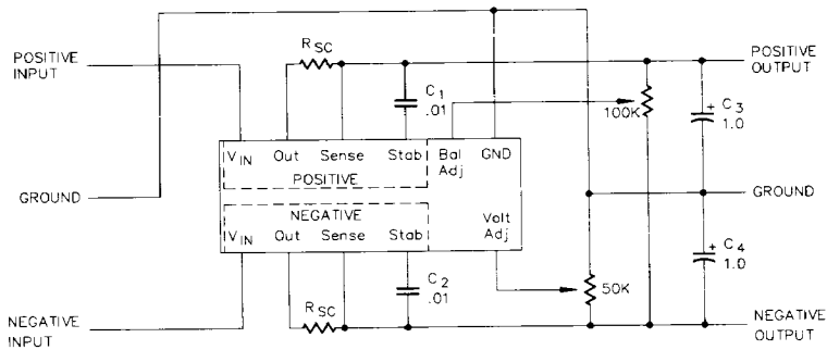
FIGURE 15 - ADJUSTMENT OF VOLTAGE LEVELS
