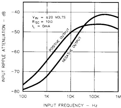
FIGURE 11. RIPPLE REJECTION
