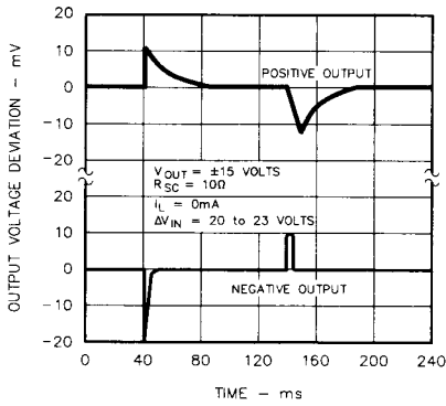
FIGURE 9. LINE TRANSIENT RESPONSE
