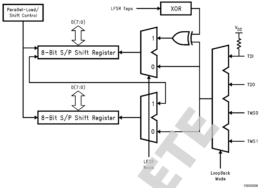
FIGURE 13. TDI Shifter/Buffer Block Diagram
