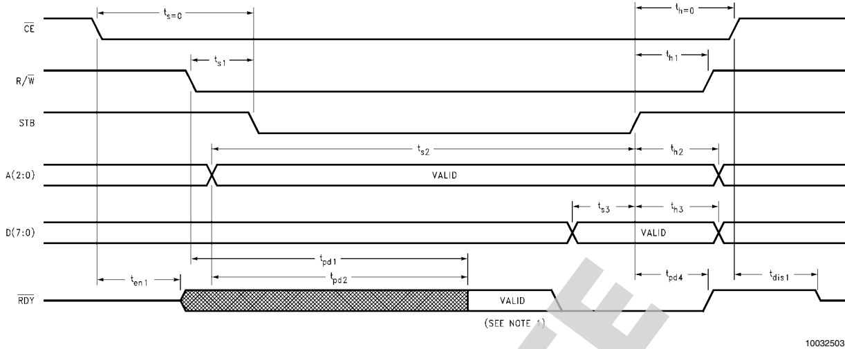
FIGURE 2. Write Cycle
