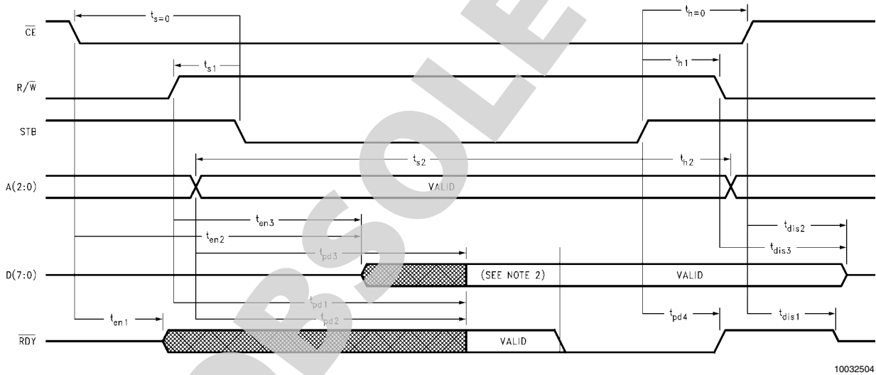
FIGURE 3. Read Cycle
