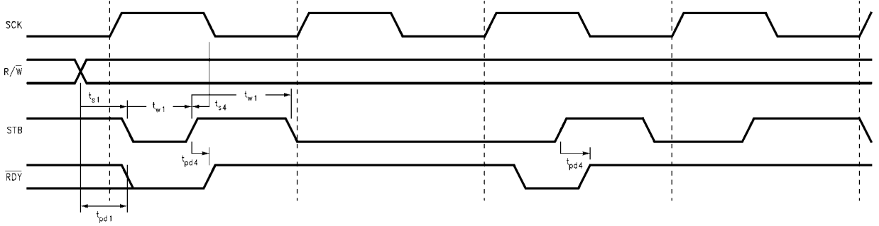
FIGURE 4. Consecutive Read/Writes (best case timing)
