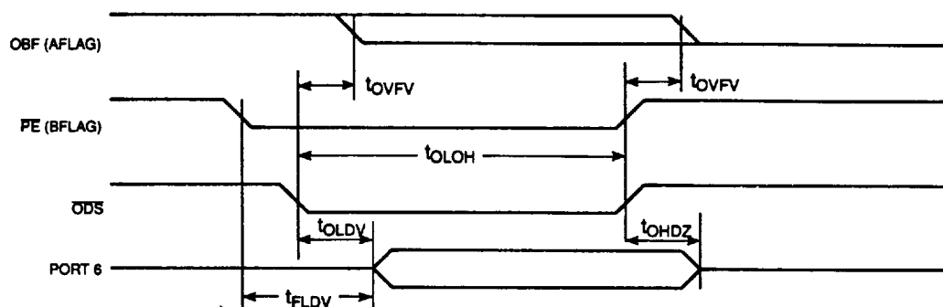
Figure 6. Port 6 Output
