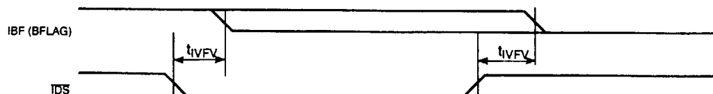
Figure 9. IBF Flag Output
