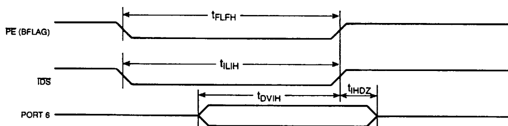
Figure 8. Port 6 Input
