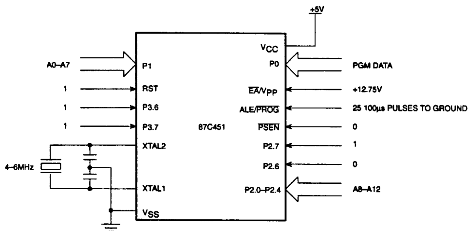
Figure 18. Programming Configuration
