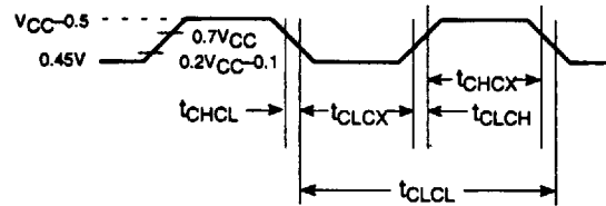
Figure 10. External Clock Drive
