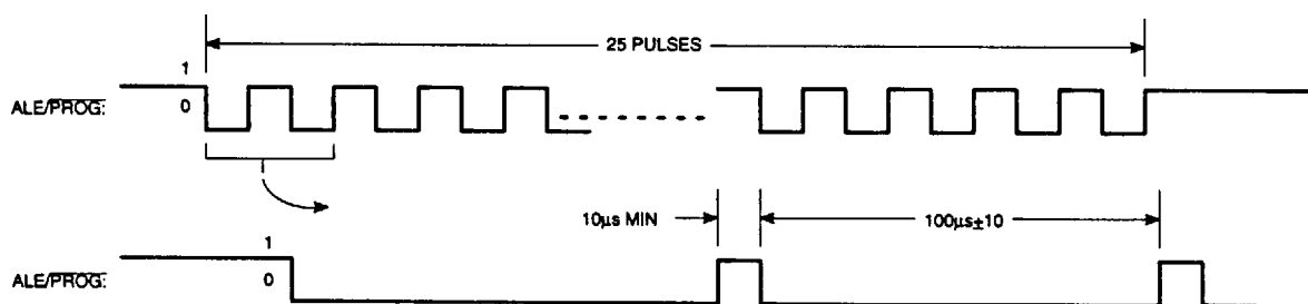
Figure 19. PROG Waveform
