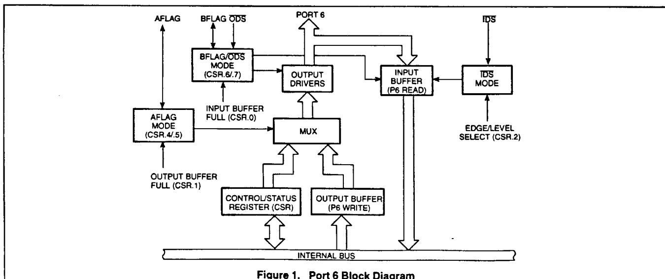
Figure 1. Port 6 Block Diagram
