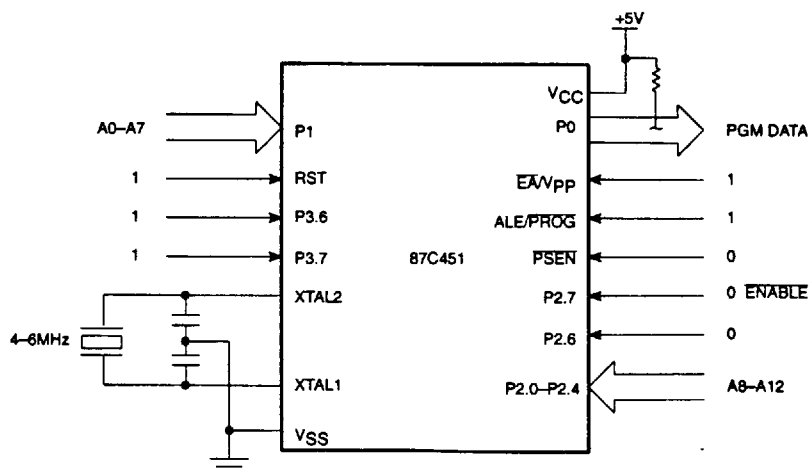
Figure 20. Program Verification
