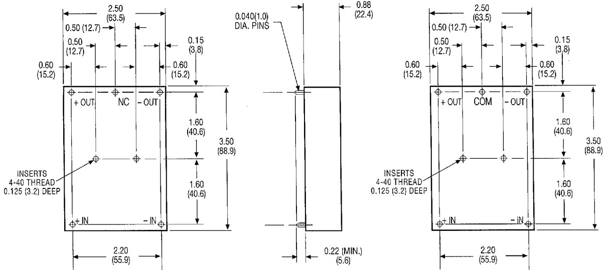
ALL DIMENSIONS INCHES (mm)
