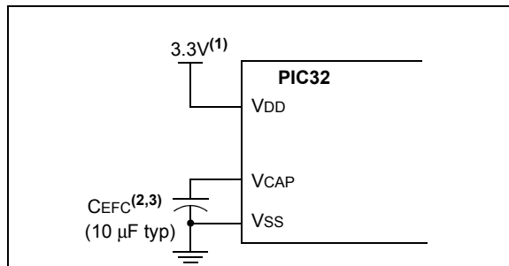
FIGURE 26-2: CONNECTIONS FOR THE ON-CHIP REGULATOR
