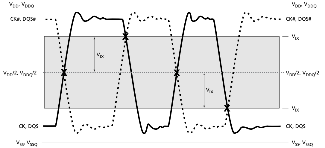
Figure 19: Single-Ended Requirements for Differential Signals
