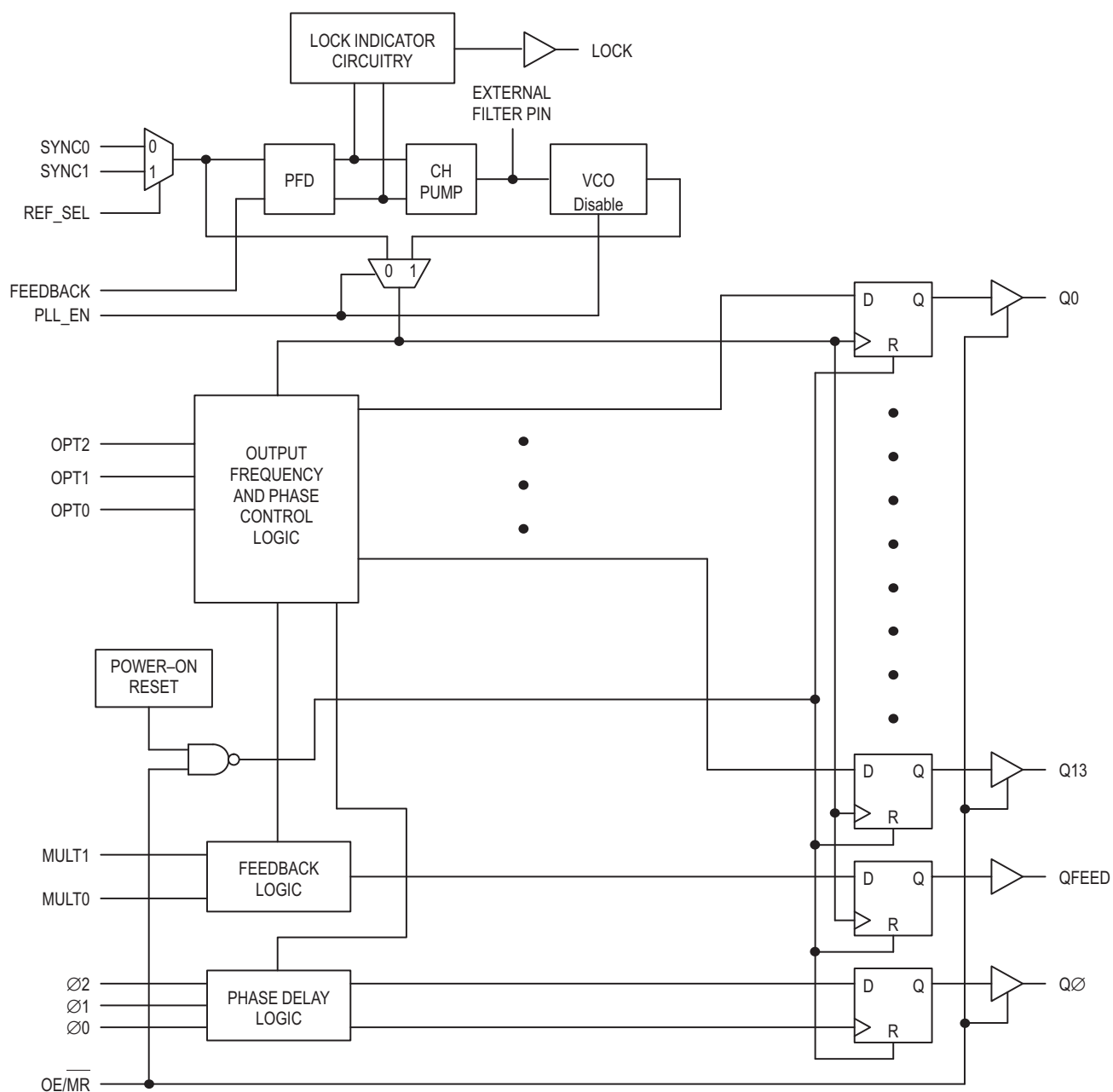
MC88PL117 Block Diagram (Logical Representation)
