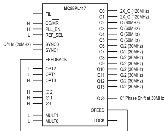
Figure 2. Output Frequency Configuration 2 (OPT0 = H, OPT1 = L, OPT2 = L) Q/4 Input Frequency, MULT0 = L, MULT1 = L)
