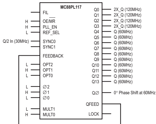
Figure 3. Output Frequency Configuration 3 (OPT0 = L, OPT1 = H, OPT2 = L) Q/2 Input Frequency, MULT0 = H, MULT1 = L)
