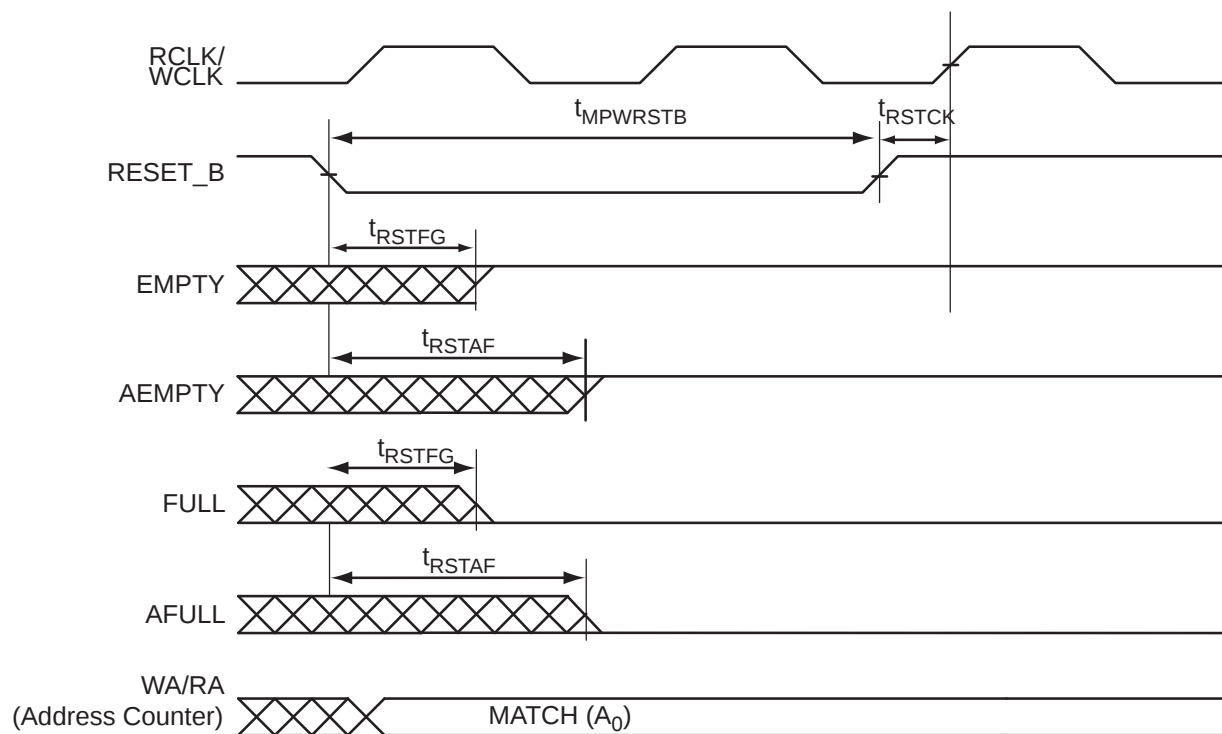
Figure 2-51 • FIFO Reset
