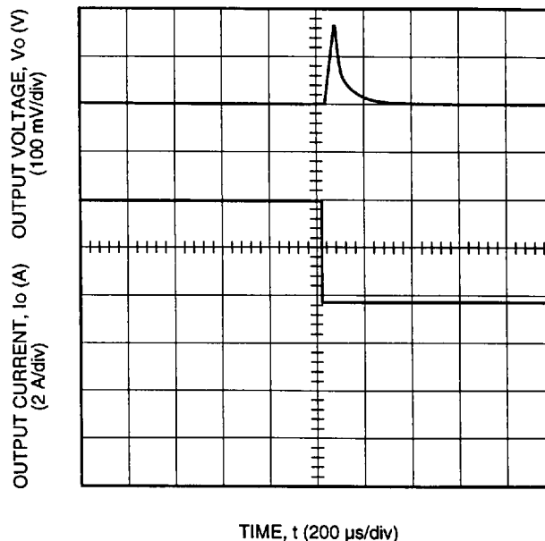
Figure 11. Typical JC100A Transient Response to Step Decrease in Load from 50% to 25% of Full Load at Room Temperature and 28 V Input (Waveform Averaged to Eliminate Ripple Component.)
