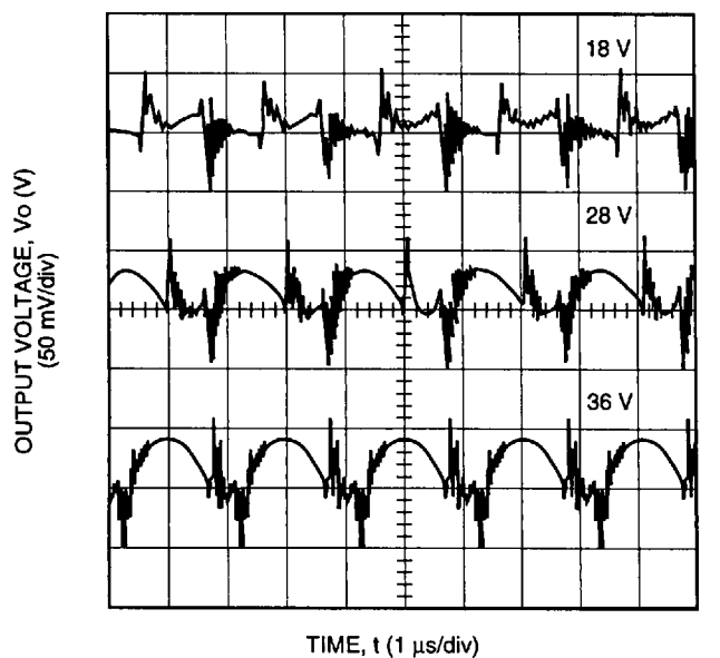
Figure 10. Typical JC100A Output Ripple Voltage at Room Temperature and 20 A Output
