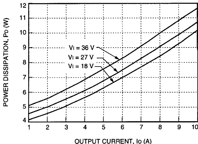
Figure 25. JC050A Power Dissipation vs. Output Current
