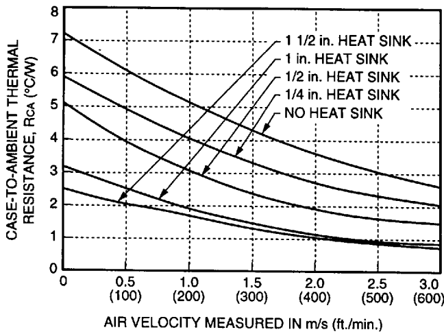
Figure 28. Case-to-Ambient Thermal Resistance Curves; Either Orientation
