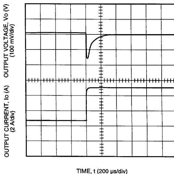
Figure 12. Typical JC100A Transient Response to Step Increase in Load from 50% to 75% of Full Load at Room Temperature and 28 V Input (Waveform Averaged to Eliminate Ripple Component.)
