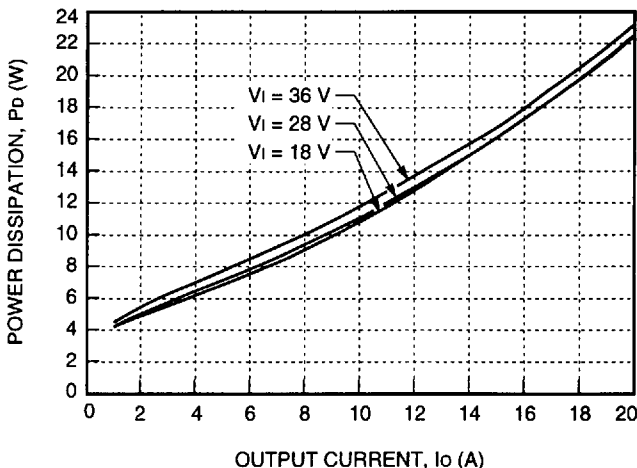
Figure 27. JC100A Power Dissipation vs. Output Current
