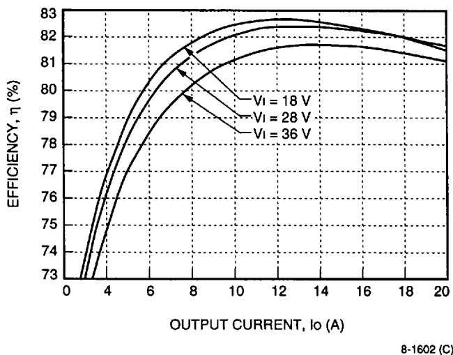
Figure 9. Typical JC100A Converter Efficiency vs. Output Current at Room Temperature
