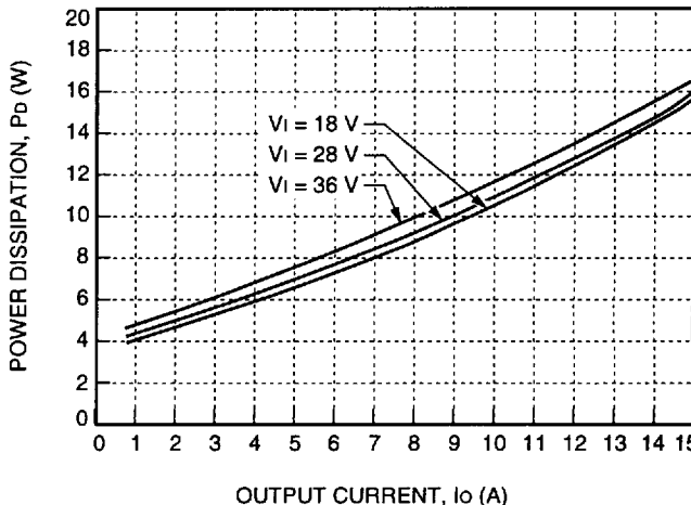
Figure 26. JC075A Power Dissipation vs. Output Current
