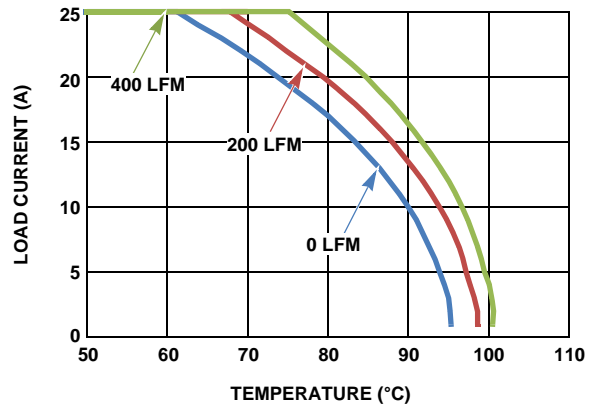
FIGURE 23. 12V_{IN} TO 3.3V_{OUT}
