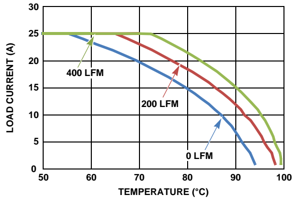
FIGURE 24. 12V_{IN} TO 5V_{OUT} , 727\text{kHz}
