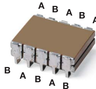
Interdigitated configuration results in reduced ESL
