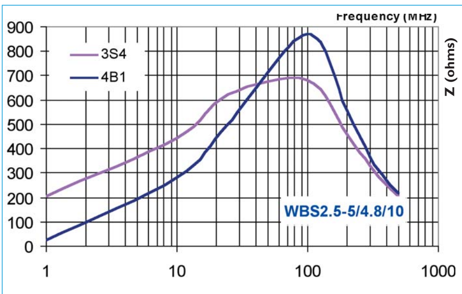
Figure 46 Z graph WBS2.5-5/4.8/10-3S4 and WBS2.5-5/4.8/10-4B1
