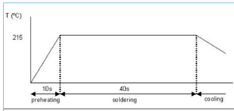
Figure 61. Vapor phase soldering
