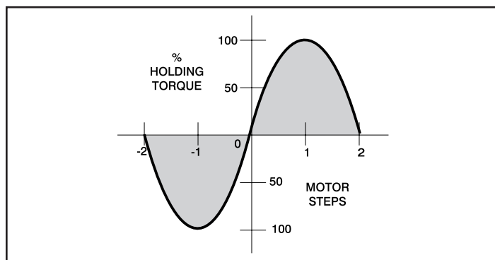
Figure 4: Torque Deflection.
