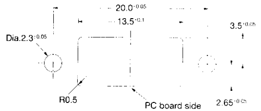
Panel Cutout
