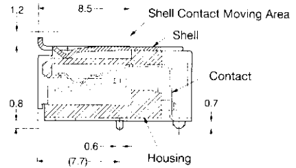
Section X-X
