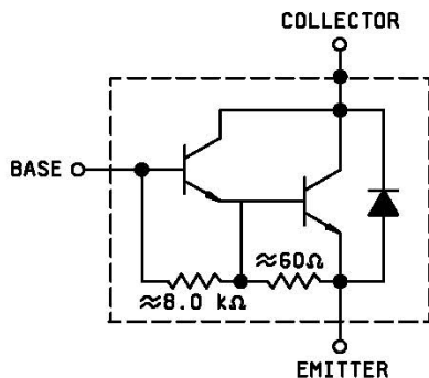
SCHMATIC CIRCUIT
